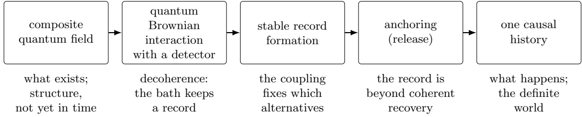
Figure 1: The backbone chain of ACT. Every statement in the theory is about one link of this chain. The first two links, and the physics of the third, are measured in the laboratory and are shared with every interpretation that keeps unitary quantum mechanics. The selection theorem (Appendix D) is ACT’s statement of the third link. The event law places the event at the fourth. The fifth is the one commitment.
